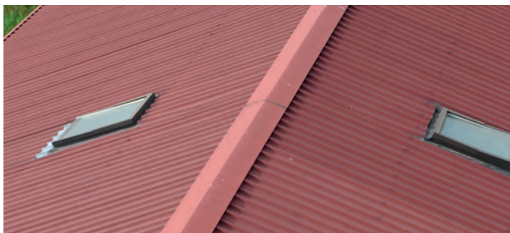
Pannelli sandwich isolpack (D5 - in alto - SUPERCOPPO in basso) Isopack's sandwich panes (D5 - above - SUPERCOPPO below)
